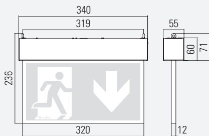
DR7E RECESSED CEILING MOUNTING
