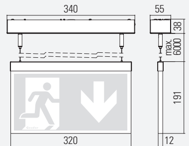
DR7S CABLE SUSPENSION MOUNTING
