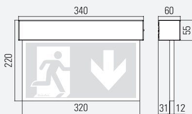
DR7Ö EYELET MOUNTING
