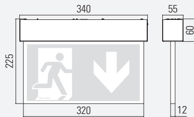
DR7A WALL BRACKET MOUNTING
