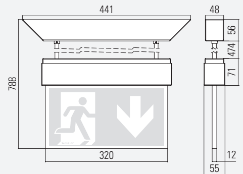
DR7S CABLE SUSPENSION MOUNTING
