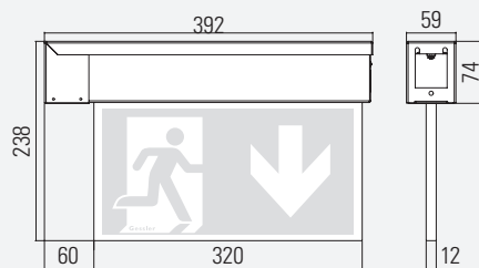
DR7F RECESSED CABLE SUSPENSION MOUNTING
