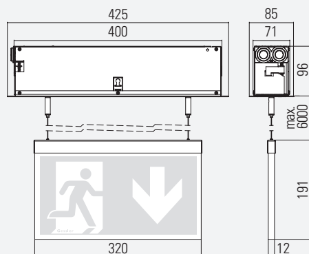
DR7F RECESSED CABLE SUSPENSION MOUNTING
